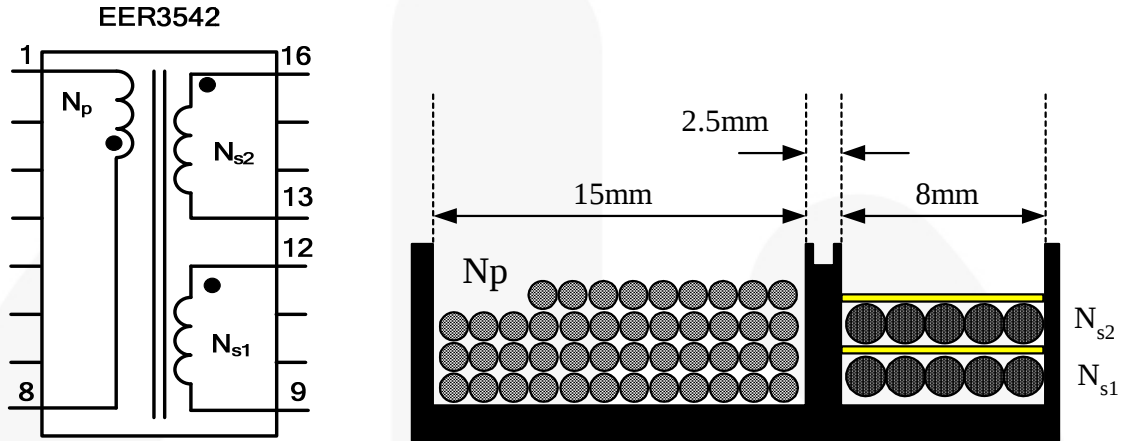
Figure 45. Winding Specifications
